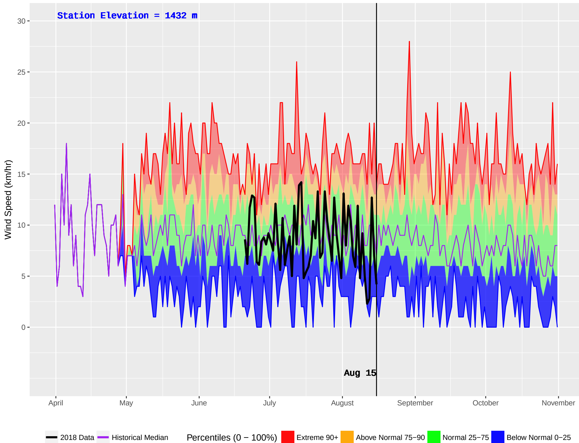
OCTOPUS CREEK (396) : Historical (2000–2016) and Current (2018) Daily Wind Speed
